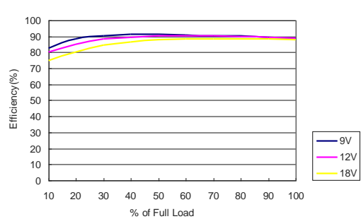
MKW40-12S15 Efficiency vs Load Current
