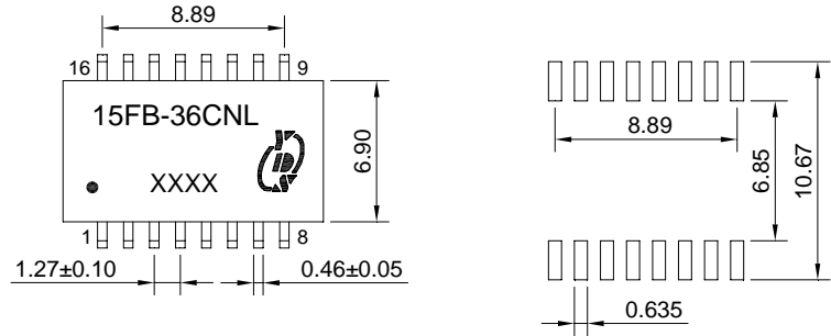
SUGGESTED PAD LAYOUT
